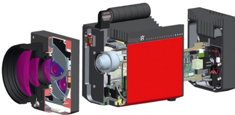
Modular system design of ImageIR ® series
